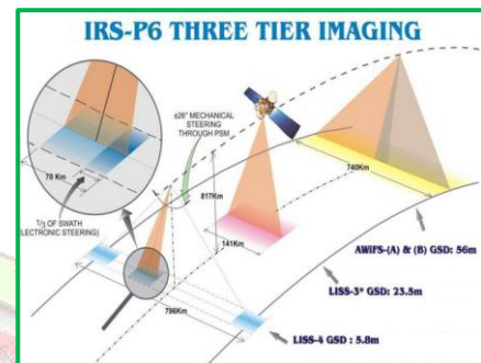
Fig. 1 Indian remote sensing platform and sensor
